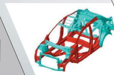
ACE™ Body Structure
